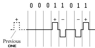
Fig. 18-4. Bipolar violation in B8ZS
